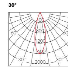
DDO075B 6W
