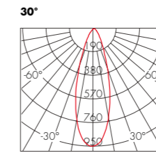
DDO075C 6W
